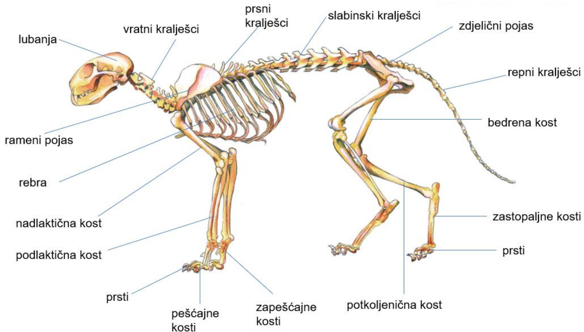
Kostur sisavaca
